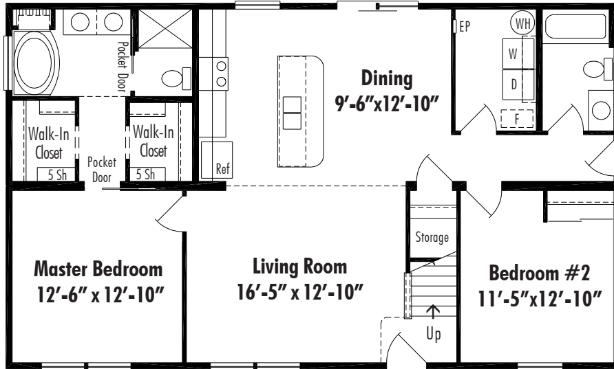
Andover III E Crawl Space 27'-4" x 46', 1257 Sq. Ft. First Floor
