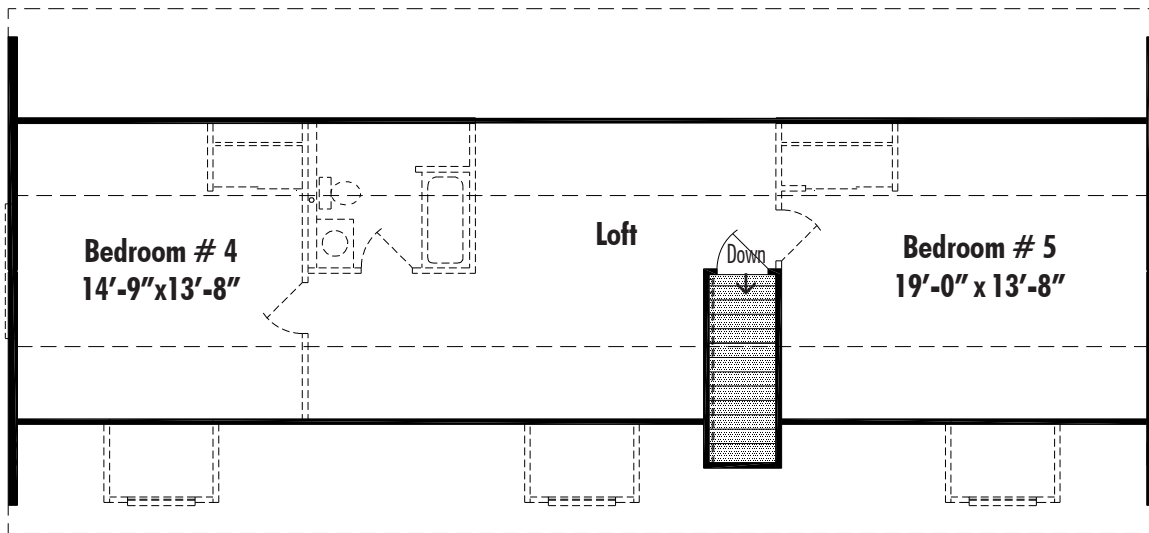
Layout A Front Stairwell 940 Sq. Ft. Second Floor
