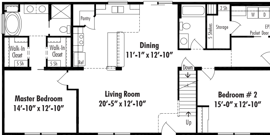
Andover I B Basement 27'-4" x 56', 1531 Sq. Ft. First Floor
