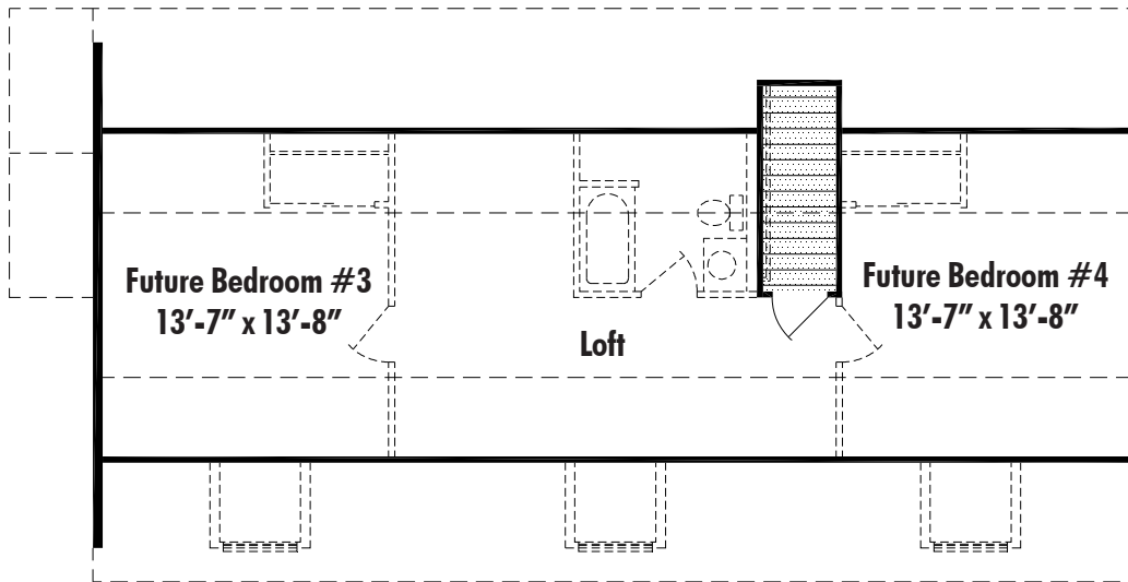
Amherst Unfinished Second Floor 27'-4" x 50', 757 Sq. Ft. Second Floor
