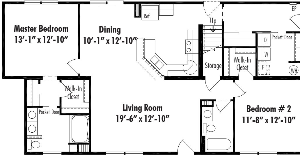
Amherst II C Crawl Space 27'-4" x 50/54' 1427 Sq. Ft. First Floor
