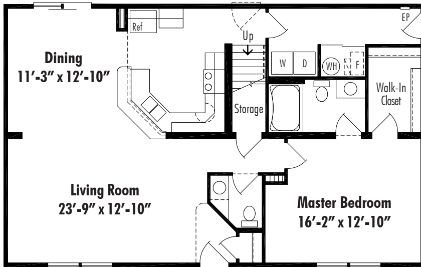
Amherst | A Crawl Space 27'-4" x 44' 1202 Sq. Ft. First Floor
