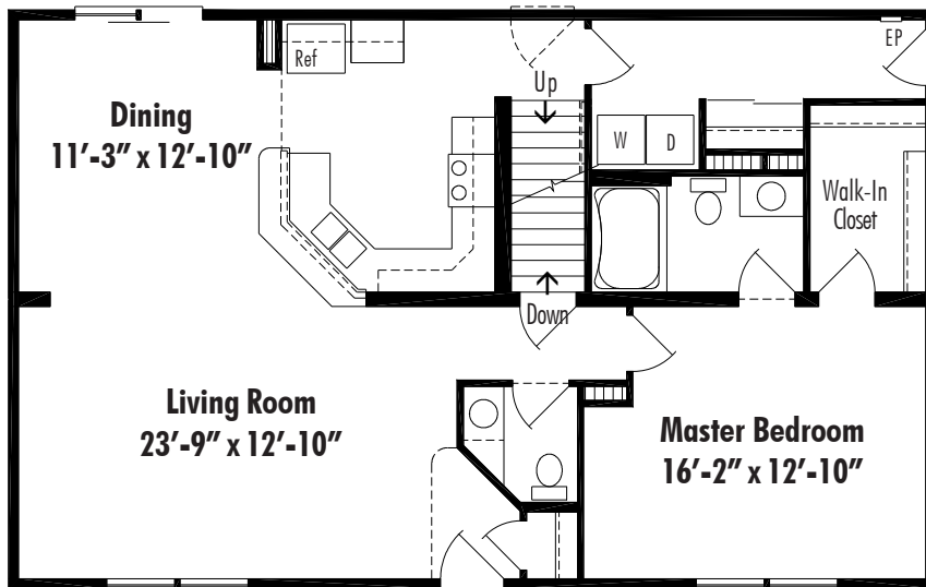
Amherst I B Basement 27'-4" x 44' 1202 Sq. Ft. First Floor
